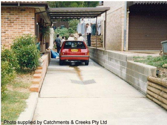
Recessed driveway & overland flow path
