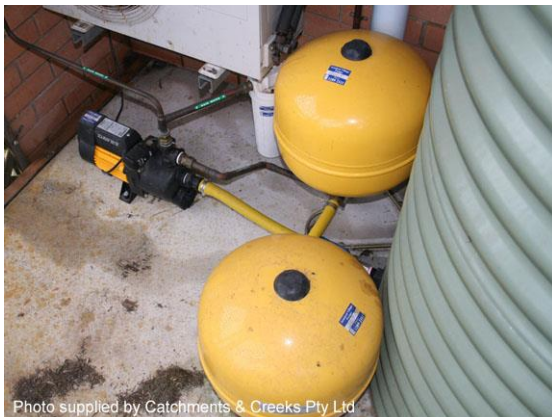
Twin (yellow) pressure tanks
