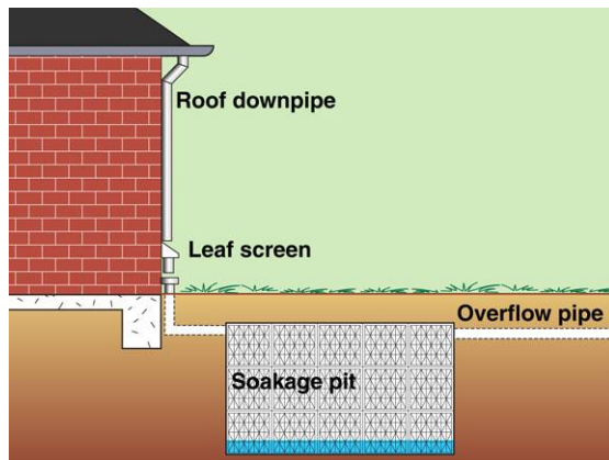
Roof water soakage pit
