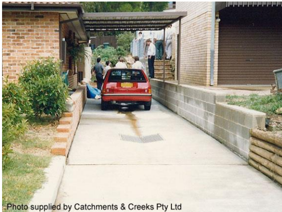
Drainage easement used as a driveway
